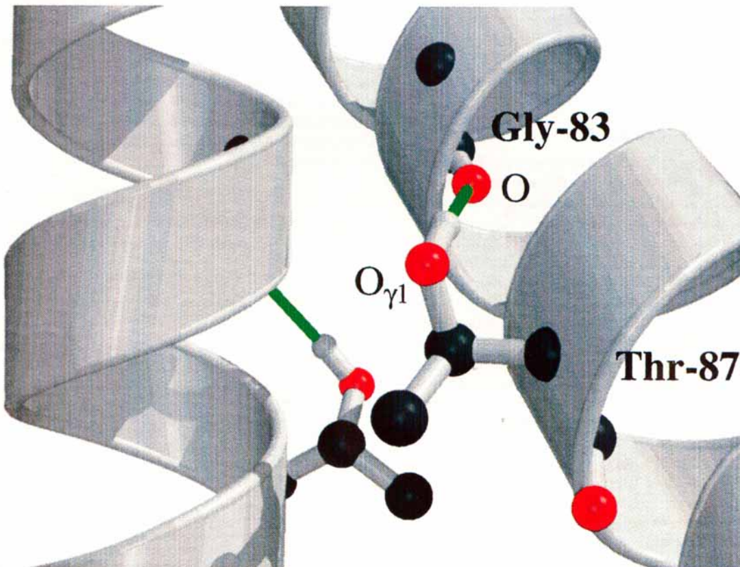
Fig. 3. The side chain to main chain hydrogen bonding observed for Thr-87 of each helix. Hydrogen bonds (shown in green) are formed between H_{\gamma 1} of Thr-87 and the main chain O of Gly-83.
