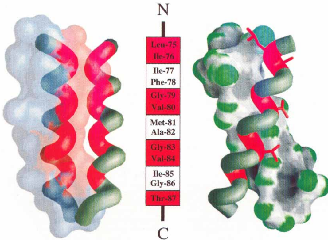
Fig. 2. The interaction between the two transmembrane \alpha -helices in the glycoprotein A dimer. In the center is the sequence encompassing the dimerization motif, the residues which are sensitive to mutation are highlighted in red throughout the figure. The leftmost image shows the highly symmetric nature of the interac-
