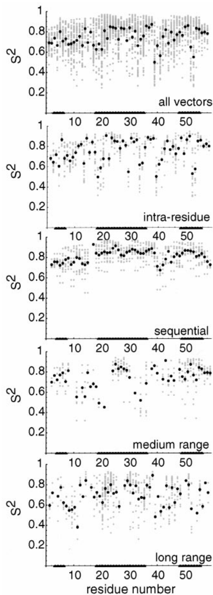
Figure 10. All order parameters \tilde{S}^2 along the sequence (grey dots) and average order parameter for each residue (black dots), for different classes of inter-proton vectors. The secondary structure is indicated by black lines in the bottom of the Figure.
