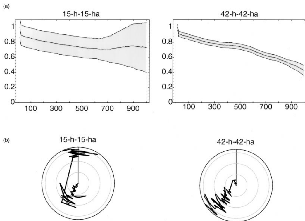
Figure 7. (a) The two intra-residue backbone-backbone correlation functions that did not converge. The shaded area corresponds to the estimated error of the correlation function (equation 15). (b) Time-series of the corresponding backbone torsion angle \phi .
