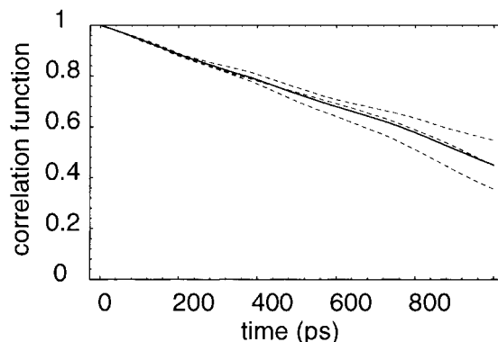
Figure 6. Correlation functions for rotational diffusion. Broken lines, three vectors rigidly attached to the protein. Continuous line, mean correlation function. The characteristic times (equation (13)) are \tau_x = 1127 , \tau_y = 1393 , \tau_z = 1711 , \langle\tau\rangle = 1355 .
