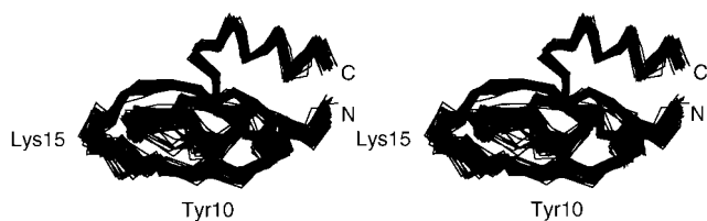
Figure 2. Snapshots of the trajectory every 100 ps.
