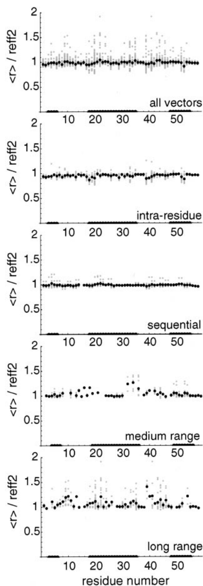
Figure 13. Ratio of \langle r \rangle / r_{\text{eff},2} for different classes of NOEs (grey dots) and the average ratio for each residue (black dots). The secondary structure is indicated by black lines in the bottom of the Figure.
