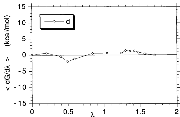
FIGURE 7. Free energy derivative with respect to \lambda for the M13Ile \rightarrow M13Ile dummy mutation in the complex, corresponding to ( \diamond ) curve d of Figure 4. \lambda represents the length of the corresponding path in Figure 4.
