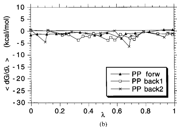
FIGURE 11. (a) Free energy derivative vs. \lambda for the M13Ile \leftrightarrow M13Val mutation in the peptide, obtained with the NL method. (b) Free energy derivative vs. \lambda for the M13Ile \leftrightarrow M13Val mutation in the peptide, obtained with the PP method.
