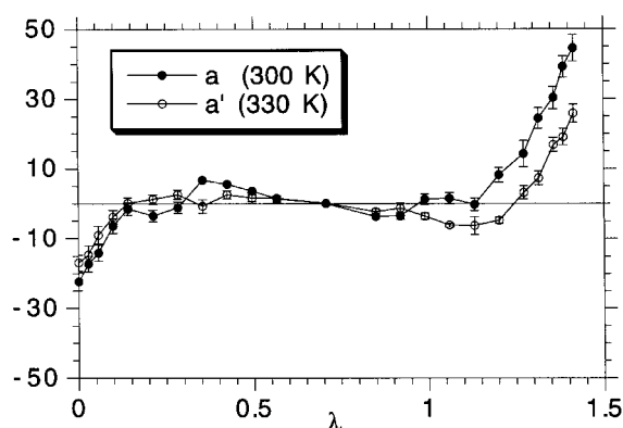
FIGURE 5. Free energy derivative with respect to \lambda for the M13Ile \rightarrow M13Ile dummy mutation in the complex, corresponding to curve a of Figure 4. (●, curve a) temperature of the restrained relaxation step T = 300 K; (○, curve a' ) temperature of the restrained relaxation step T = 330 K. \lambda represents the length of the corresponding path in Figure 4.
