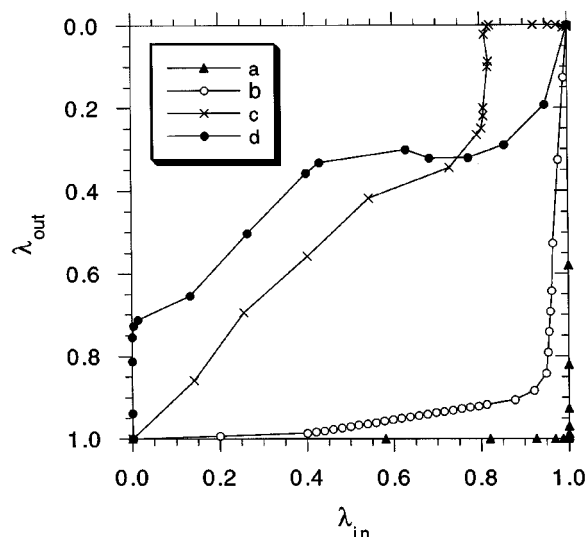
FIGURE 8. Path of the different M13Ile \leftrightarrow M13Leu mutations of the peptide in the \lambda_{in}, \lambda_{out} plane. (Curve a) NL method using eq. (6) with r_1 = r_2 = 0.07 ; (curve b) NL + SPM methods with two independent parameters, \lambda_{in} and \lambda_{out} , for the forward mutation; (curves c, d) PP + SPM methods with two independent \lambda_{in} and \lambda_{out} for forward and backward mutations, respectively.
